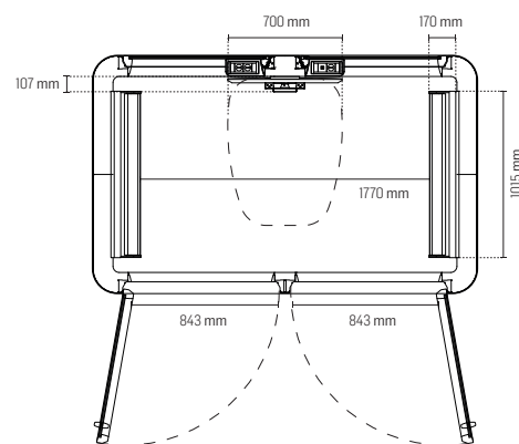
With 2x retractable sofas:
